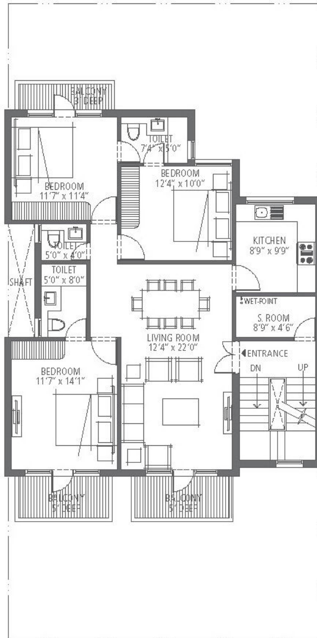
First & Second Floor Plan
